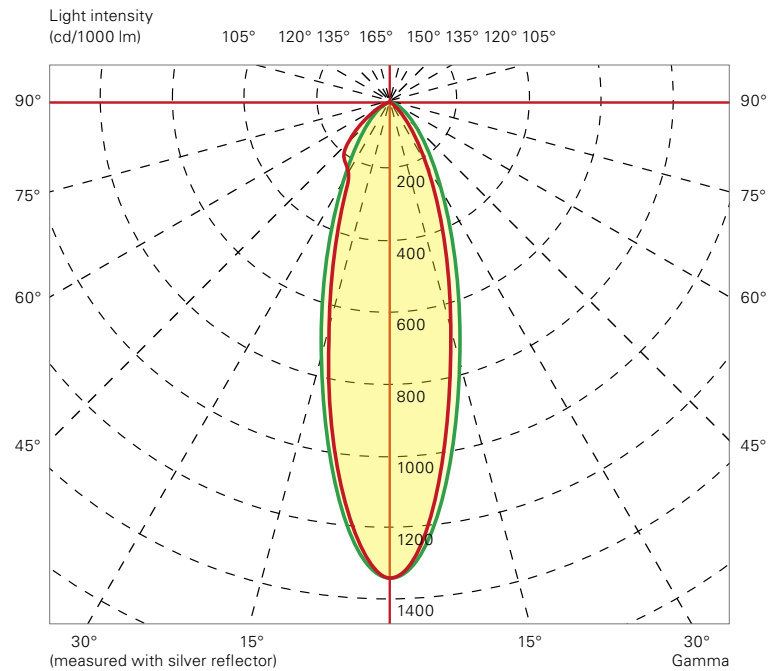
WallBeam reflector (BBS 100 W)
