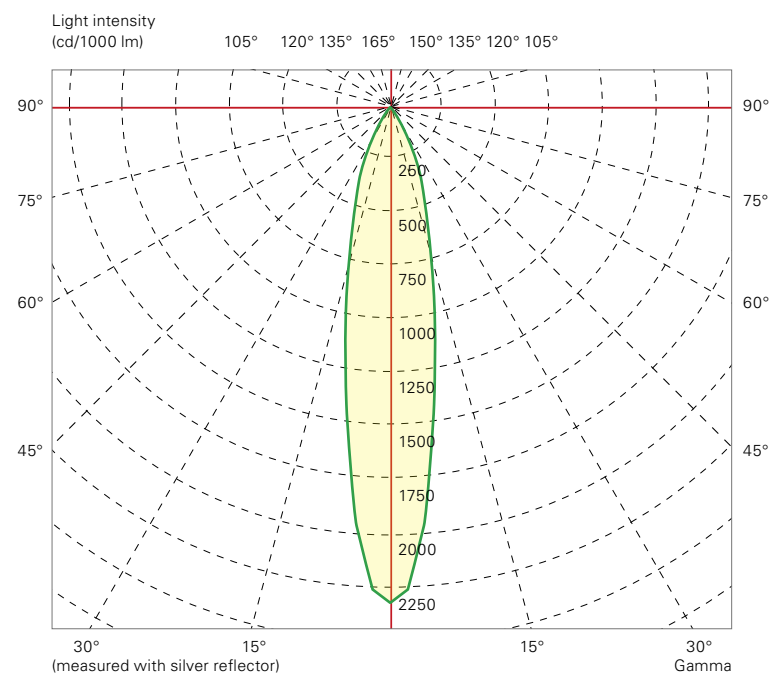
Spot reflector (BBS 100 W)
