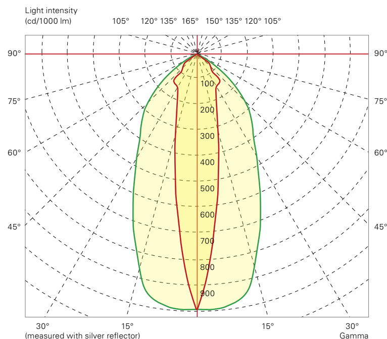
MaxBeam reflector (BBS 100 W)
