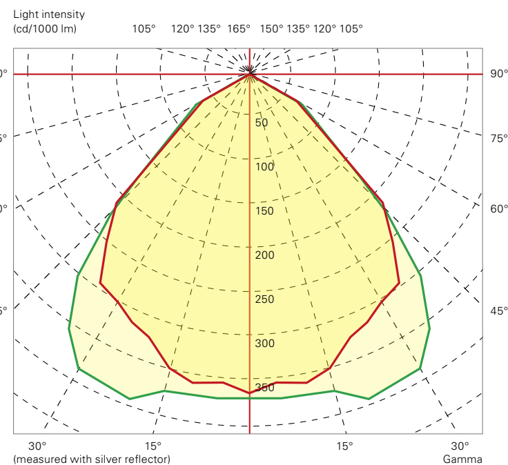
Flood reflector (BBS 100 W)
