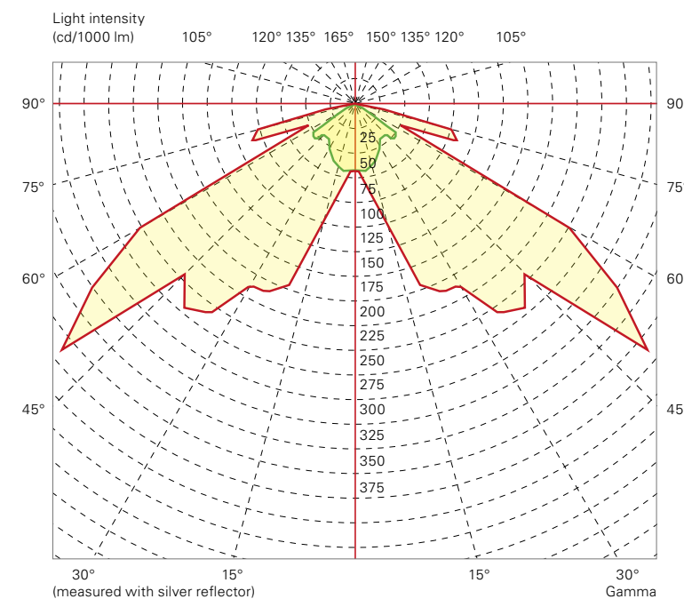
Batwing reflector 90° (BBS 100 W)
