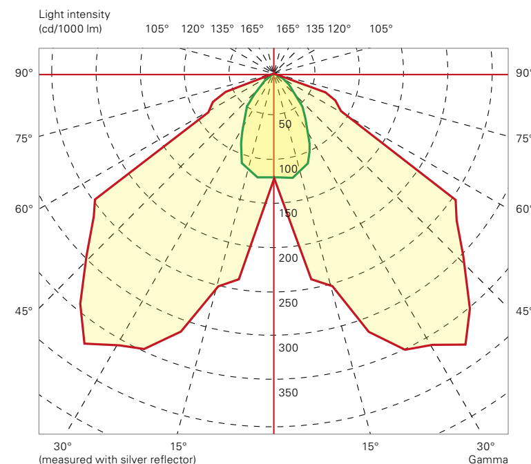
Batwing reflector 70° (BBS 100 W)
